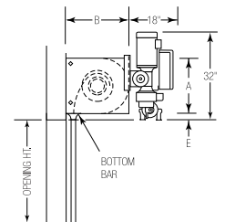
MOTOR (GEARHEAD) SECTION
